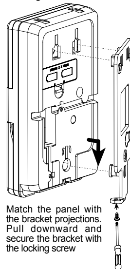
Figure 6: Panel Mounting
