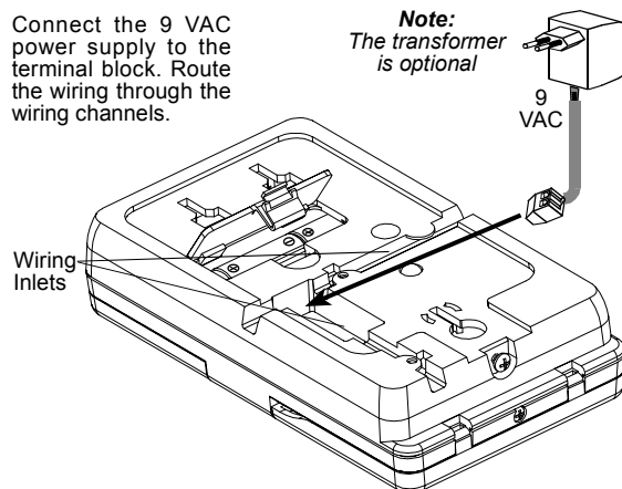
Figure 5: Wiring
